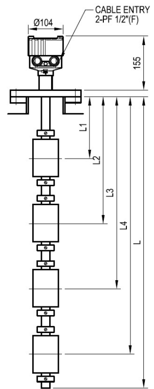
HR-30V-Ex
