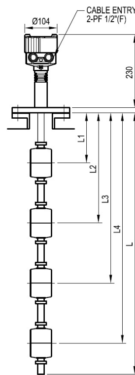
HR-30SH-Ex
