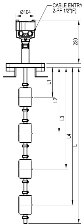
HR-30SH-Ex
