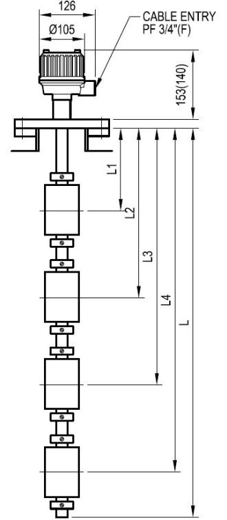
HR-30V
