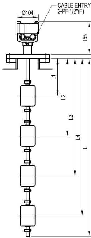
HR-30S-Ex
