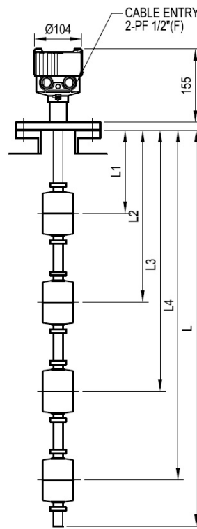
HR-30T-Ex
